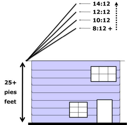
Slope: 8:12 + Roof Height: 25' + Slide Guards CAN'T BE USED for Fall Protection
